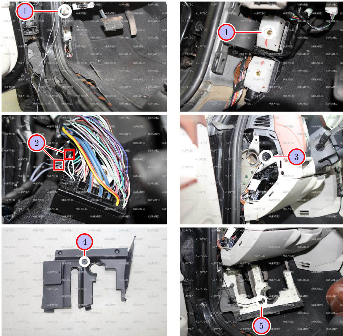
Figure 6: Connection Can High & Low / Installation pushbutton
