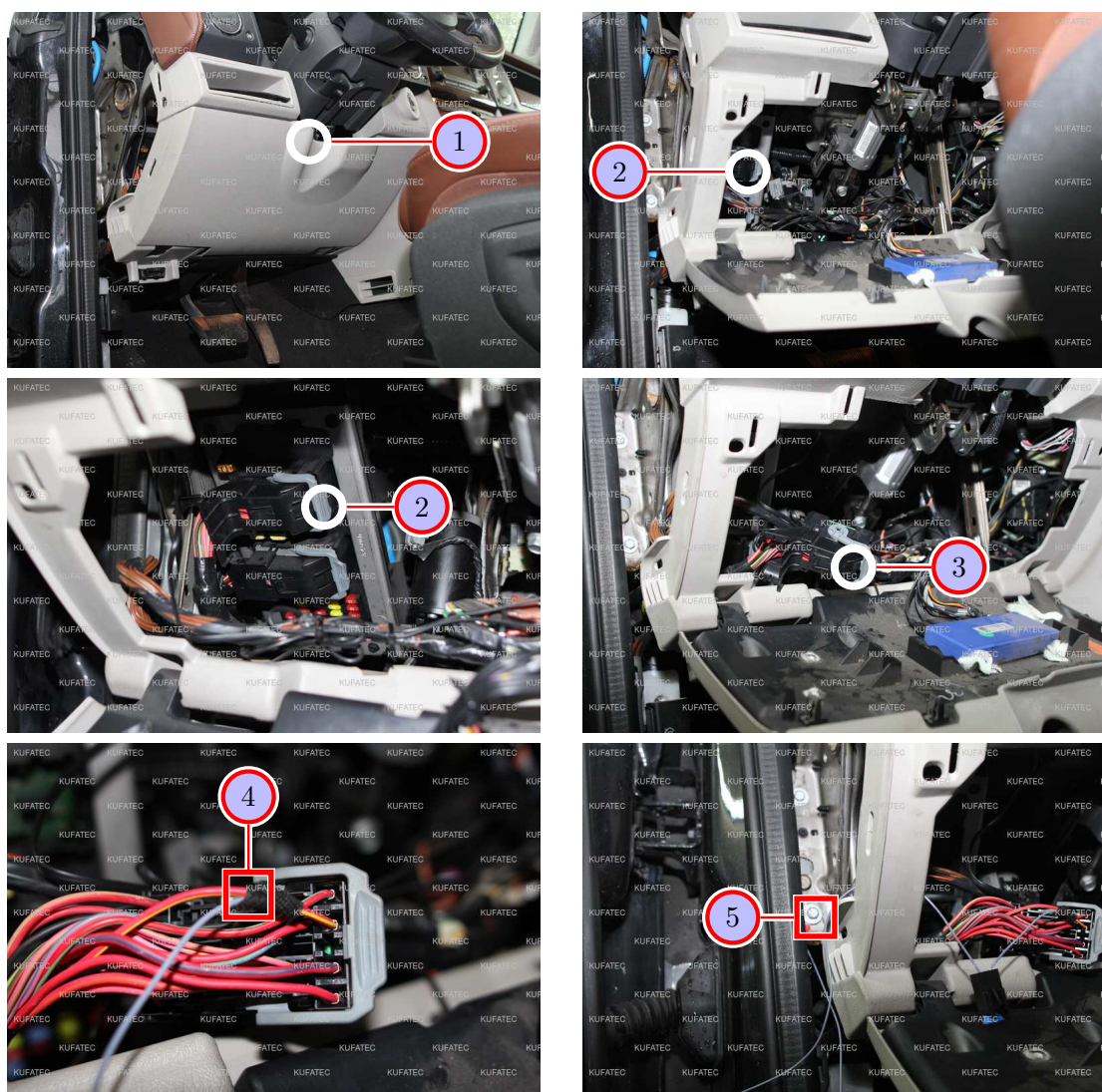
Figure 5: Connection ignition lead / ground
