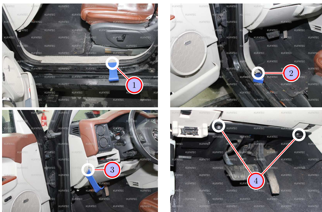
Figure 4: Removing trim panel driver's side
